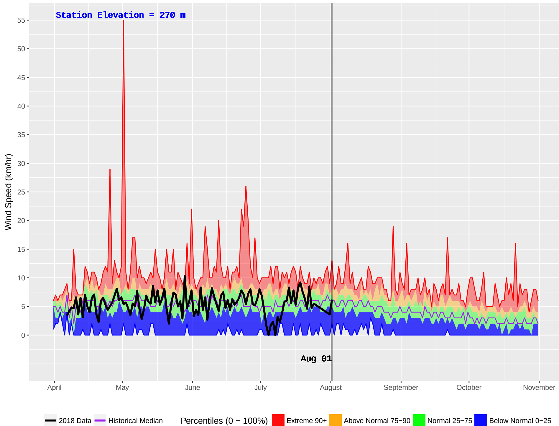
TALCHAKO (233) : Historical (1990–2016) and Current (2018) Daily Wind Speed
