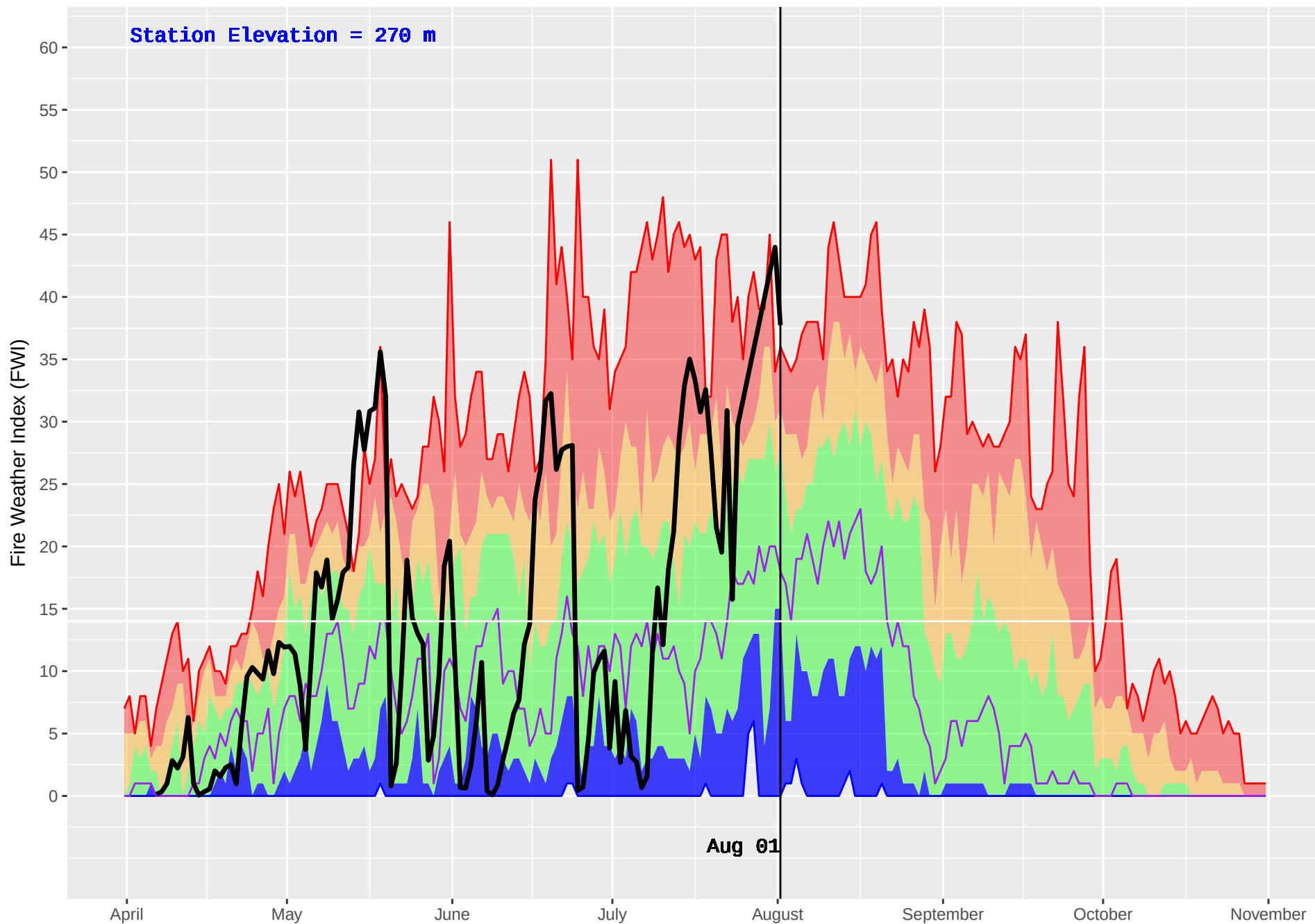
TALCHAKO (233) : Historical (1990–2016) and Current (2018) Daily Fire Weather Index (FWI)
