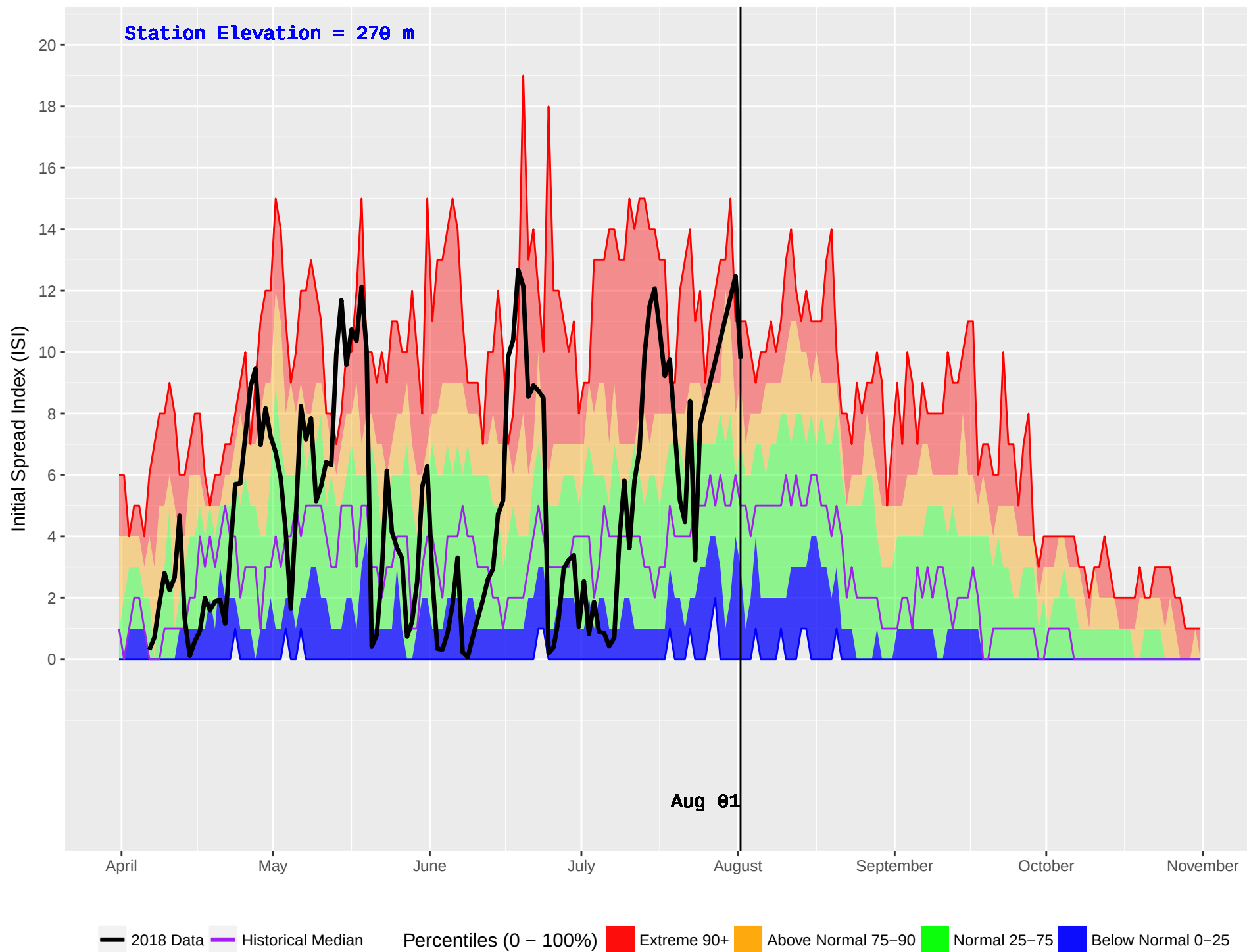
TALCHAKO (233) : Historical (1990–2016) and Current (2018) Daily Initial Spread Index (ISI)
