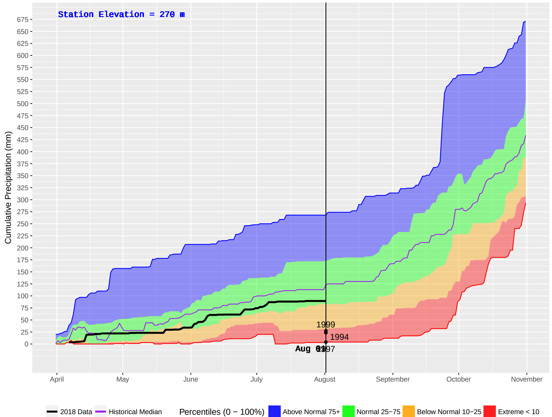
TALCHAKO (233) : Historical (1990–2016) and Current (2018) Daily Cumulative Precipitation
